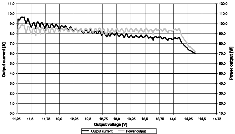
EFOY Pro 2400: U-I and U-P characteristic
