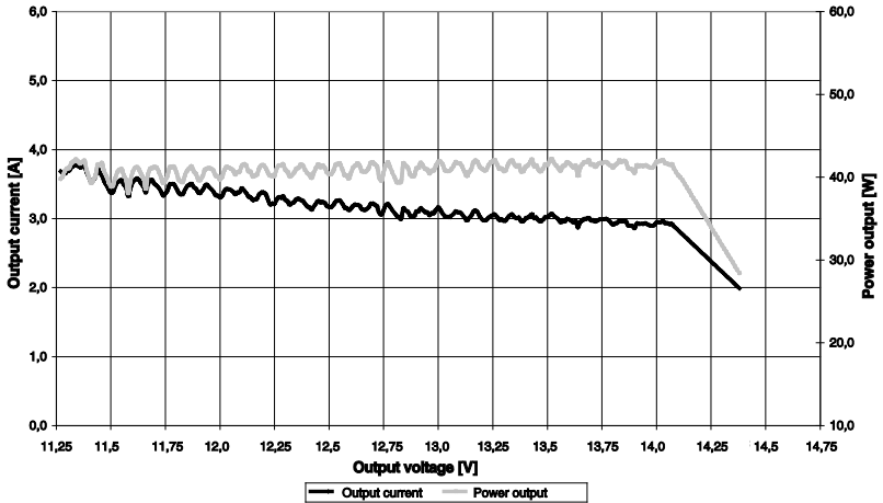
EFOY Pro 800: U-I and U-P characteristic
